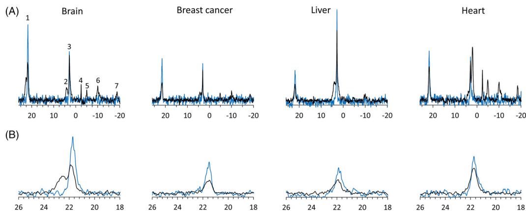
FIGURE 1 Phosphorus-31 nuclear magnetic resonance ( ^{31}\text{P} -NMR) spectra acquired from ex vivo preparations of perfused brain slices, breast cancer slices, liver slices, and retrograde perfused heart. (A) Blue: spectra of the perfusion media for the various tissues supplemented with 3-aminopropylphosphonate (3-APP) (without the tissue). Black: spectra of the viable tissues perfused with these media. (B) Expansion of the 3-APP signal of the spectra shown in (A). Only the spectrum of the brain slices shows an additional signal, upfield to the 3-APP signal of the perfusion medium. Each spectrum was recorded using a flip angle of 50^\circ , TR of 1.1 s, and 5740 averages (total scan time of 105 min). Signal assignment: 1, 3-APP; 2, phosphomonoesters, 3, inorganic phosphate; 4, phosphocreatine; 5, \gamma -adenosine triphosphate ( \gamma -ATP); 6, \alpha -ATP; 7, \beta -ATP
