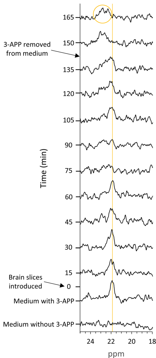
FIGURE 2 Demonstration of 3-aminopropylphosphonate (3-APP) accumulation in the rat brain slices. Representative ^{31}\text{P} spectra of 3-APP signal over time in the course of a wash-in/wash-out experiment. From the bottom up: the medium only (without brain slices) devoid of 3-APP; supplementation of 3-APP to the same medium; time 0 is the time at which the brain slices were introduced to the NMR tube; after 135 min, 3-APP was washed out of the perfusion system by replacing the perfusion medium with a medium that did not contain 3-APP. The yellow straight line indicates the position (in ppm) of the 3-APP m signal; the yellow circle highlights the 3-APP b signal (bound to the brain slices). Each spectrum was recorded using a flip angle of 50^\circ , TR of 1.1 s, and 820 averages (total scan time of 15 min)
