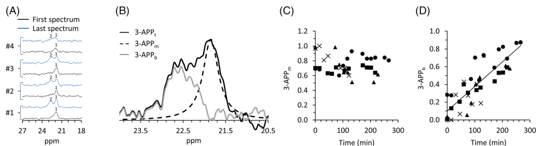
FIGURE 3 Accumulation of 3-aminopropylphosphonate (3-APP) in the brain. (A) Accumulation of 3-APP in brain slices from four different rats. For each animal (#1 through 4), the spectrum in black shows the 3-APP t signal at the beginning of the incubation of the slices with 3-APP, and the signal in blue shows the 3-APP t at the end of the incubation period. The 3-APP m and 3-APP b components of the 3-APP t signal are denoted as 1 and 2, respectively. The spectra were acquired with 820 scans, within 15 min each. (B) A typical 31 P signal of 3-APP t acquired from rat brain slices perfused with a medium containing 3-APP (1 mM). The acquired signal is shown in solid black; a Lorentzian lineshape fitting to the 3-APP m signal is shown with a dashed line; the result of subtracting 3-APP m signal from the 3-APP t signal is shown in gray and comprises the 3-APP b signal. The spectrum was recorded using a flip angle of 50°, a TR of 1.1 s, and 820 averages (total scan time of 15 min). (C and D) Changes in the 3-APP m and the 3-APP b signals, respectively, with perfusion time. The levels of the 3-APP m and 3-APP b signals were normalized to the 3-APP signal of the medium alone on each experimental time course ( n = 4, each experimental time course is marked with a different marker type) recorded at the beginning of each experiment. The trend line in D demonstrates the increase with time of the 3-APP b signal ( R 2 = 0.7)
